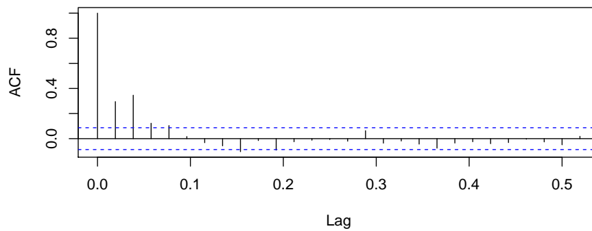
Series residuals(reg2)
